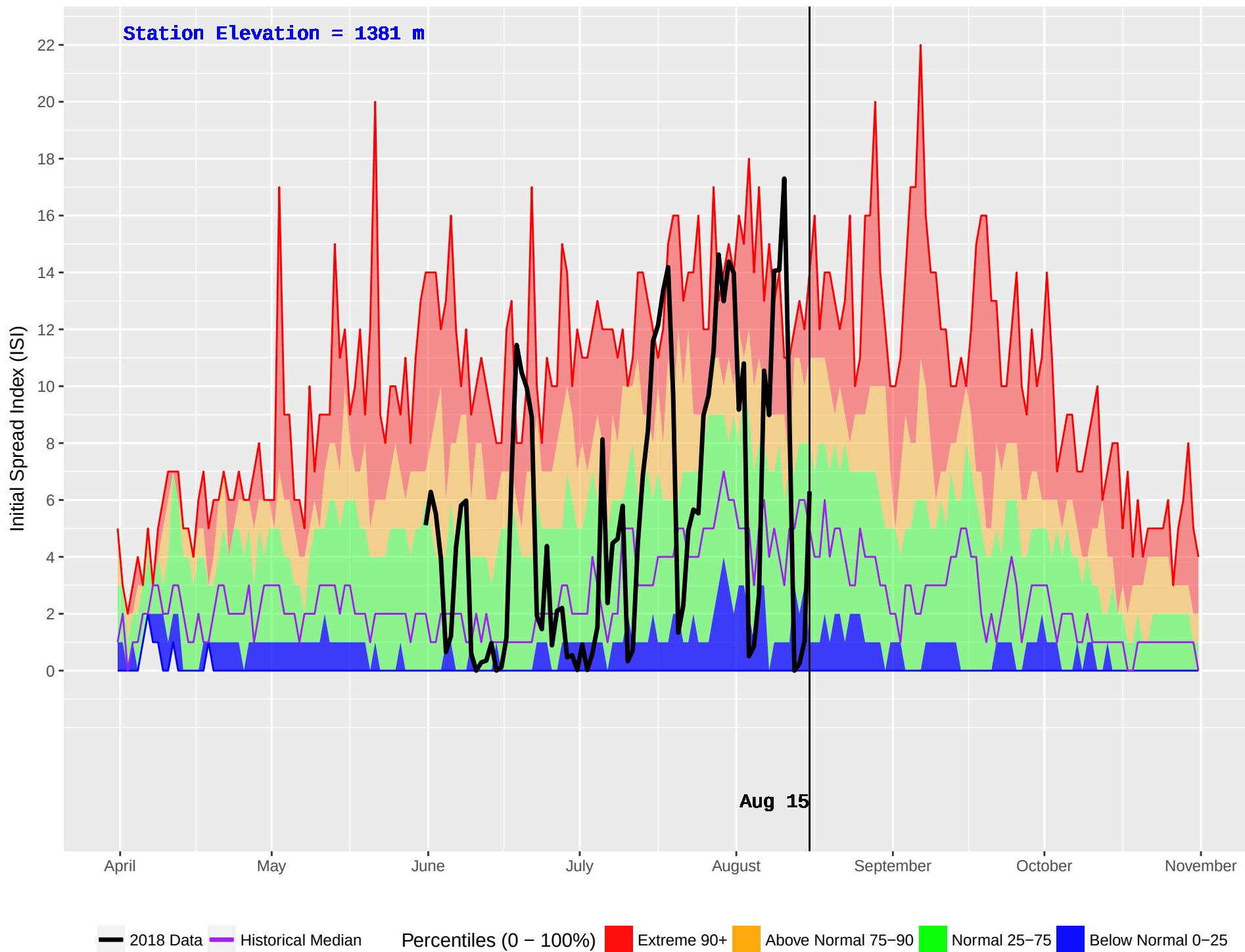
GLIMPSE (291) : Historical (1978–2016) and Current (2018) Daily Initial Spread Index (ISI)
